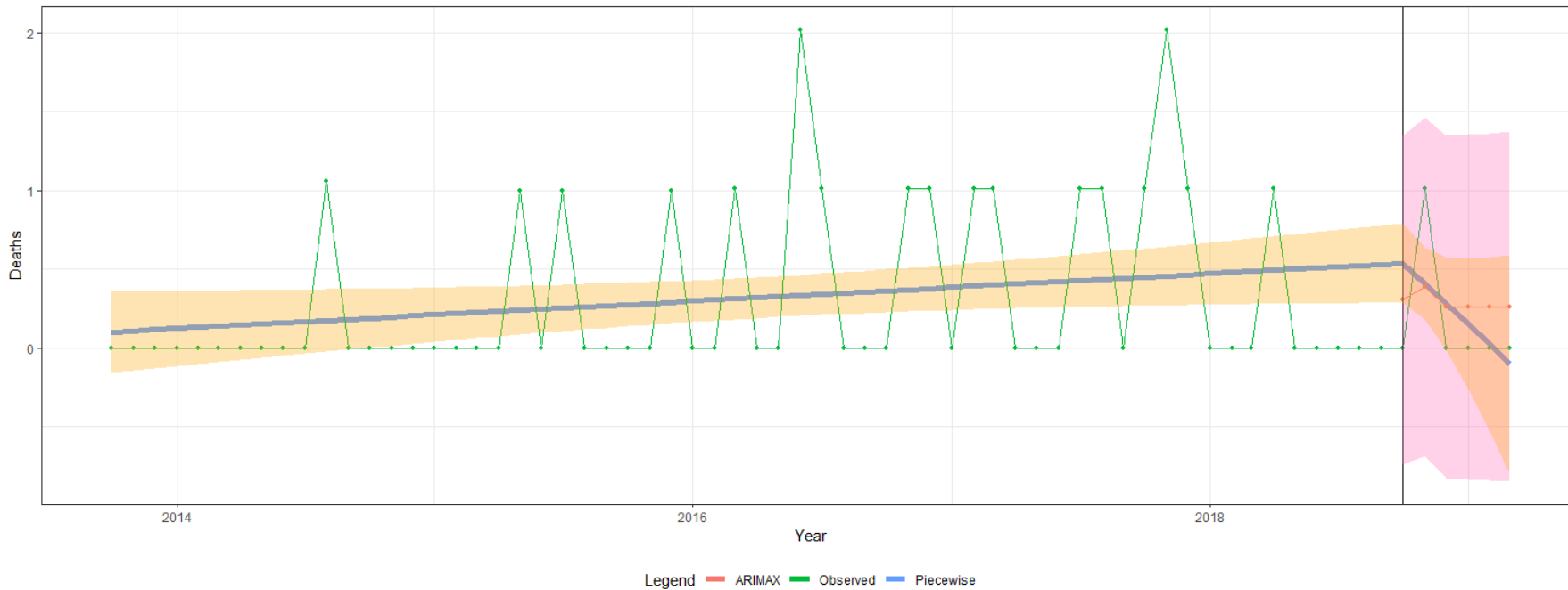
Supplemental Figure 4. Red Deer Opioid-related Deaths. Piecewise 95% CI in Orange, ARIMAX 95% CI in Pink. Intervention On 2018-10-01
